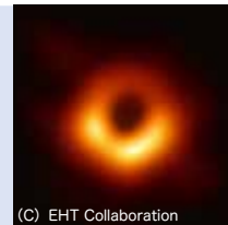
(C) EHT Collaboration
